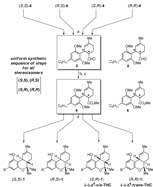
Scheme 2. Stereodivergent preparation of all stereoisomers of Δ 9 -THC (1). Reagents and conditions: a) Grubbs II cat. (3 mol %), CH 2 Cl 2 , 25 °C, 92% for (S,S)-5, 87% for (R,S)-5, 90% for (S,R)-5, 85% for (R,R)-5; b) NaClO 2 (2.3 equiv), NaH 2 PO 4 (2.0 equiv), 2-methyl-2-butene (30 equiv), tBuOH/H 2 O, 25 °C; c) Me 3 SiCHN 2 (1.1 equiv), C 6 H 6 /MeOH (1:1), 0 °C, 66% for (S,S)-6, 60% for (R,S)-6, 61% for (S,R)-6, 65% for (R,R)-6; d) MeMgI (10 equiv), Et 2 O, 0 °C to 160 °C, ambient pressure to 150 mm Hg; then addition of ZnBr 2 upon workup in CH 2 Cl 2 , 25 °C, 57% for (S,S)-6, 41% for (R,S)-6, 45% for (S,R)-6, 65% for (R,R)-6. R = C 5 H 11 . Atom numbering in the nomenclature of 1 (shown in Figure 1 a) has been dropped for clarity; thus, (S,S)-1 is (6aS,10aS)-1, and so on.
